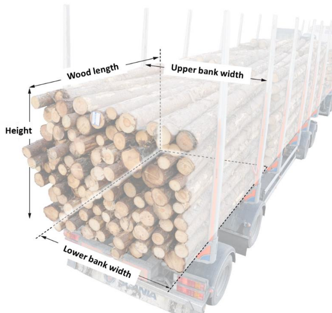
Figure 1. Measurement of stack on a vehicle.
